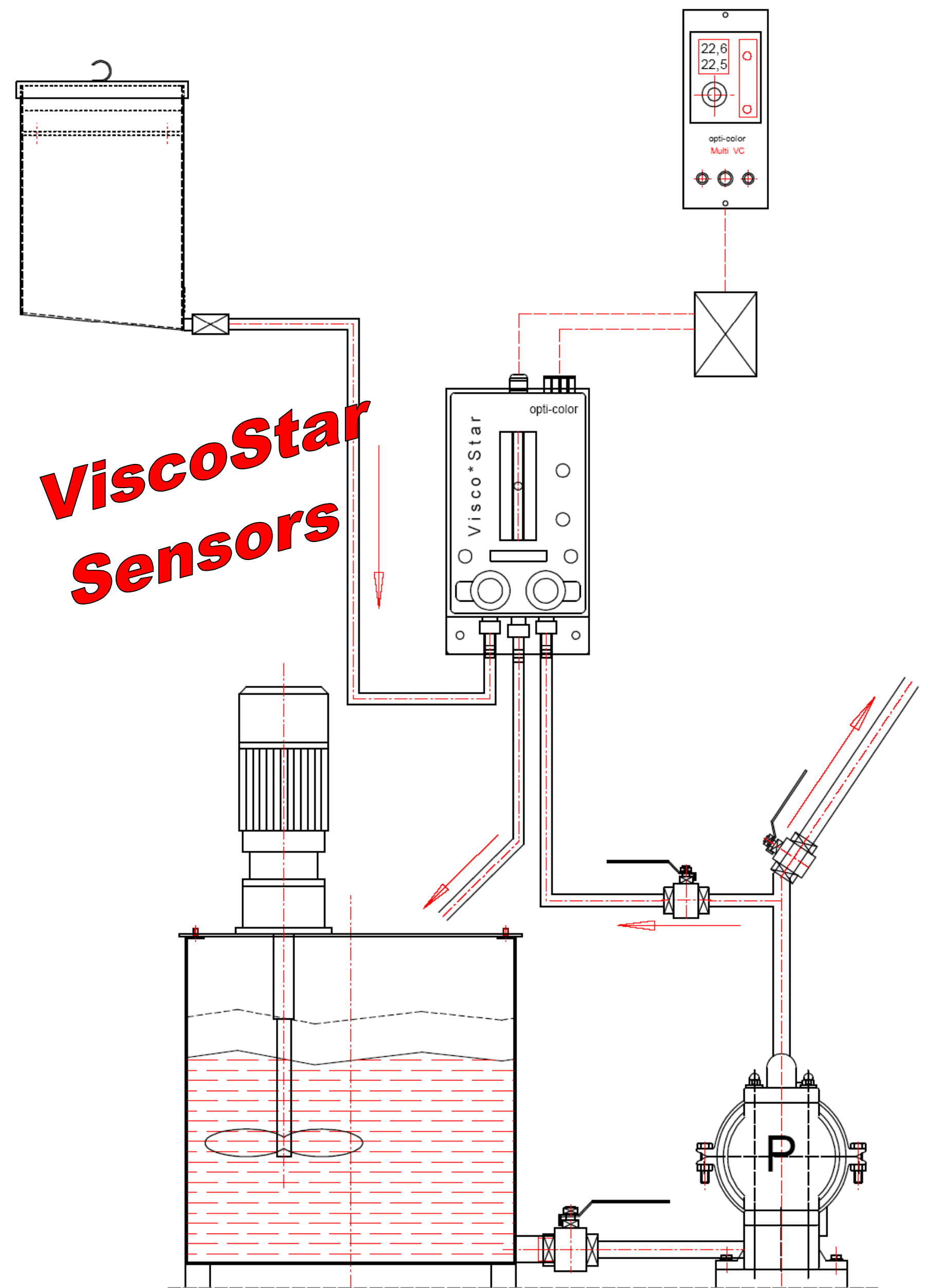
Falling Ball Sensor in Bypass
