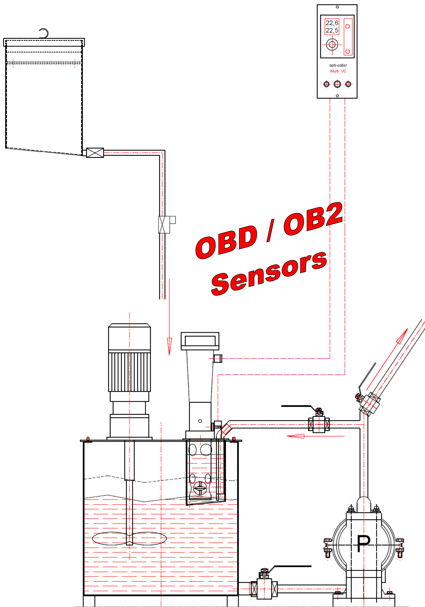
Rotating Sensor in Tank/Bypass
